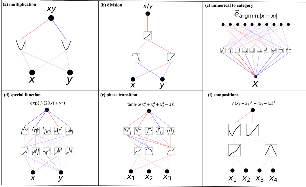
Figure B.2: LANs on synthetic examples. LANs do not appear to be very interpretable. We conjecture that the weight matrices leave too many degree of freedoms.
